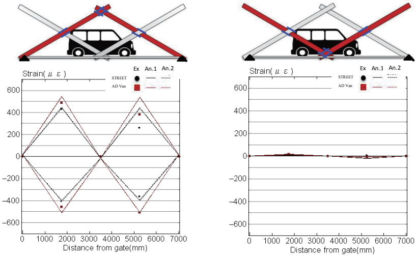
(a) Structural members of ends-support (b) Structural members with free ends
