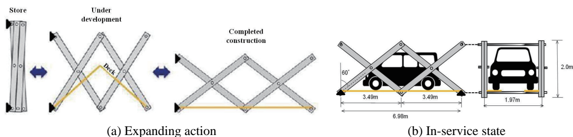
Figure 1: Outline of the experimental MB1.0
