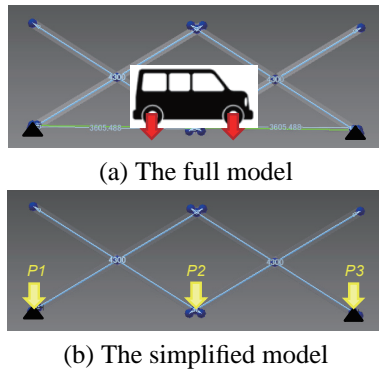
Figure 2: Outline of the 2D model as a simple support
